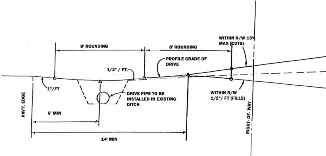
Figure 6 Driveway Details
